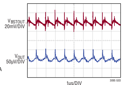
Output Ripple
